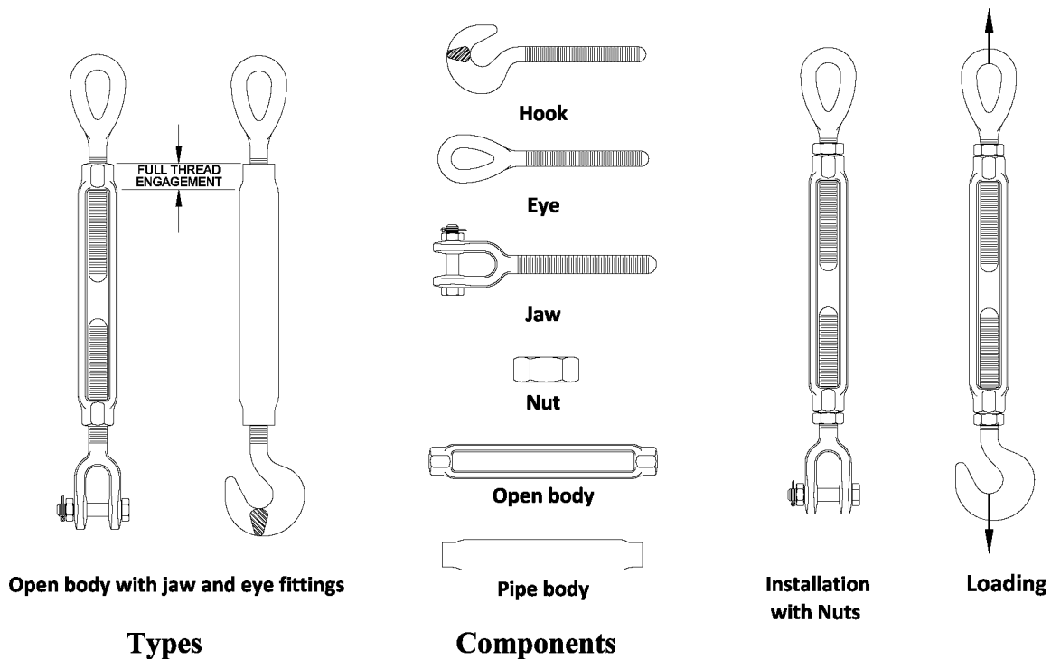
Figure 30 Turnbuckle Types
